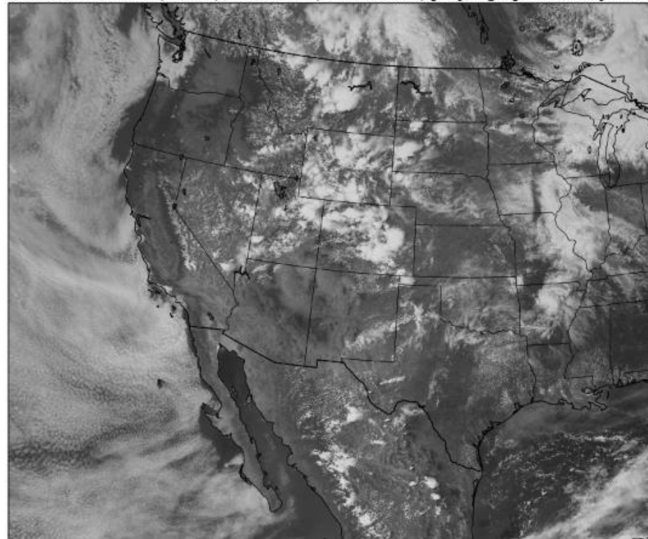
GOES-16 Channel 2 (visible) / Channel 7 (shortwave IR) [Day/Night] at 20:55Z Jun 14,
