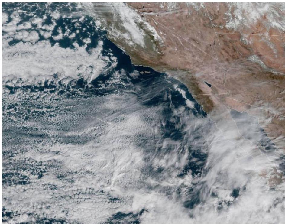
14 Jan 2020 20:00Z NOAA/NESDIS/STAR GOES-West ABI GEOCOLOR
