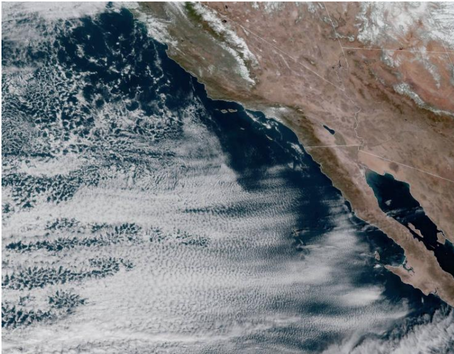
13 Jan 2020 20:00Z NOAA/NESDIS/STAR GOES-West ABI GEOCOLOR
