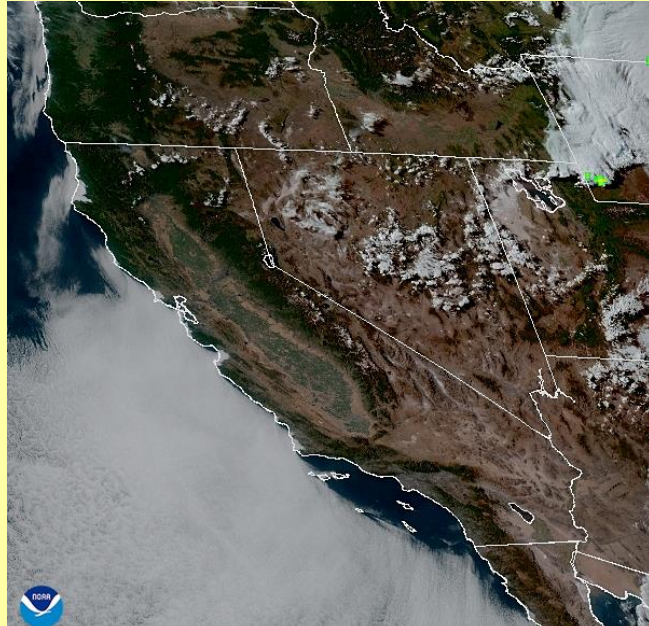
22 Jun 2024 01:31 NESDIS/STAR GOES-West GLM FED
