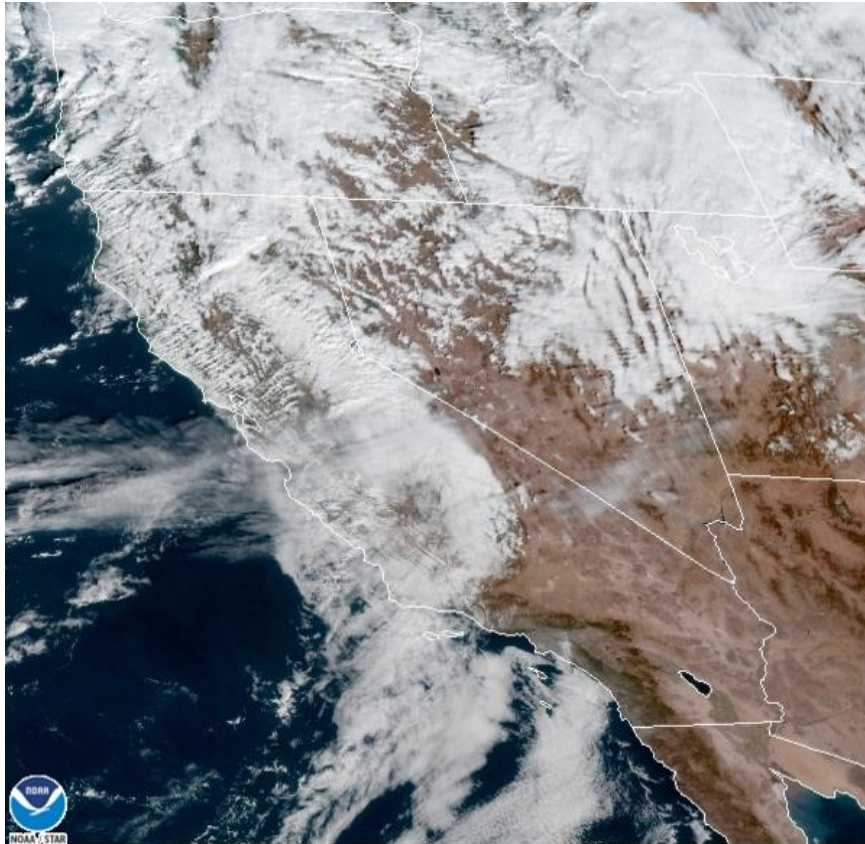
18 Nov 2020 18:46Z NESDIS/STAR GOES-West GEOCOLOR
